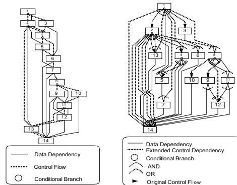
(a) Macro Flow Graph (MFG) (b) Macro Task Graph (MTG)
