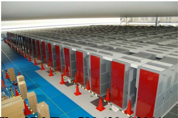
The 27th Top 500 (20.6.2011), No.1 , Fujitsu "K" 548,352 cores (Current Peak 8.774 PFLOPS) LINPACK 8.162 PFLOPS (93.0%)
